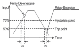
3) Lo alarm & Energised relay
